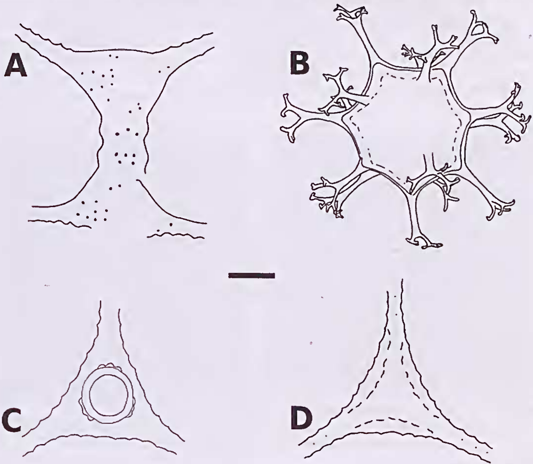
Figure 3. Line drawings of Staurostrum sp. from Baroon Pocket Dam. A. Ornamentation of basal inflation; B. Zygospore; C. Annulus, showing shape and ornamentation; D. Apex, showing intramarginal verrucae. Scale Bar = 10 \mu\text{m} .
